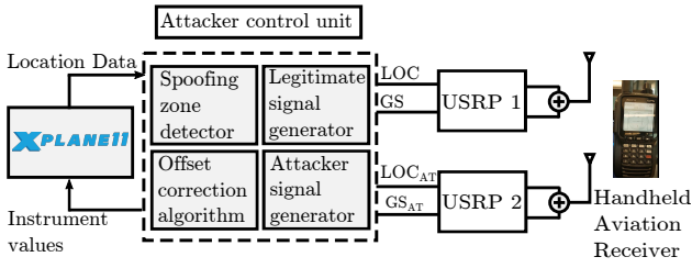
Figure 2: Schematic of the experiment setup used for evaluating the attacks on ILS.
