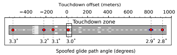
Figure 5: Results of glideslope spoofing.
