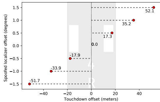
Figure 4: Results of localizer spoofing.
