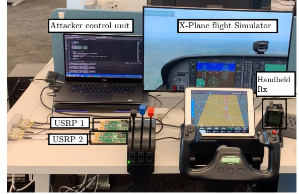
Figure 3: Photo of the experiment setup.
